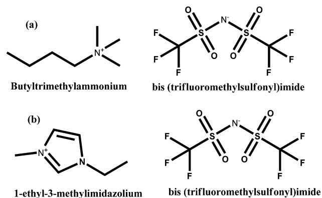
Scheme 1 Structures of (a) [BMAMm + ][TFSI – ] and (b) [EMIm + ][TFSI – ]
