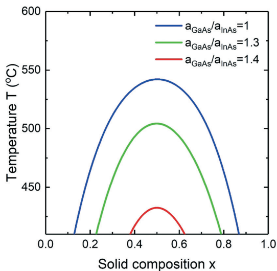
Fig. 5 The miscibility gap in \text{In}_x\text{Ga}_{1-x}\text{As} alloy at c_{\text{As}} = 0.01 for different surface energy ratios.
