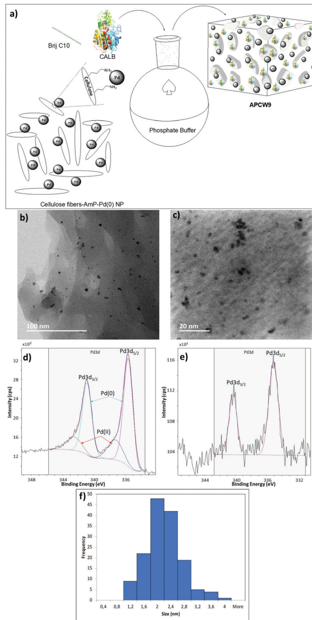
Fig. 2 (a) Fabrication of APCW9. TEM images of APCW9, (b) scale bar 100 nm and (c) scale bar 20 nm. XPS spectra of Pd 3d 5/2 for (d) MCC-Amp-Pd(0) and (e) APCW9 (that had been stirred for 24 h in toluene, at 90 °C, under H 2 atmosphere). (f) Size distribution of the Pd nanoparticles of APCW9.
