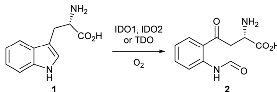
Scheme 1 Dioxygenation of L-tryptophan 1 to N-formyl-L-kynurenine 2 .
