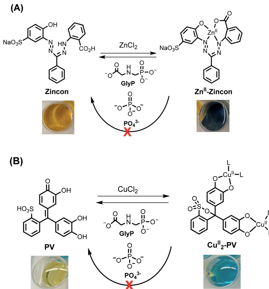
Fig. 4 Schematic representation and changes of the color of reactions between \text{Zn}^{\text{II}} -zincon (30 \mu\text{M} ; (A)) or \text{Cu}_2^{\text{II}} -PV (30 \mu\text{M} ; (B)) and GlyP (10 equiv.) or \text{PO}_4^{3-} (10 equiv.).
