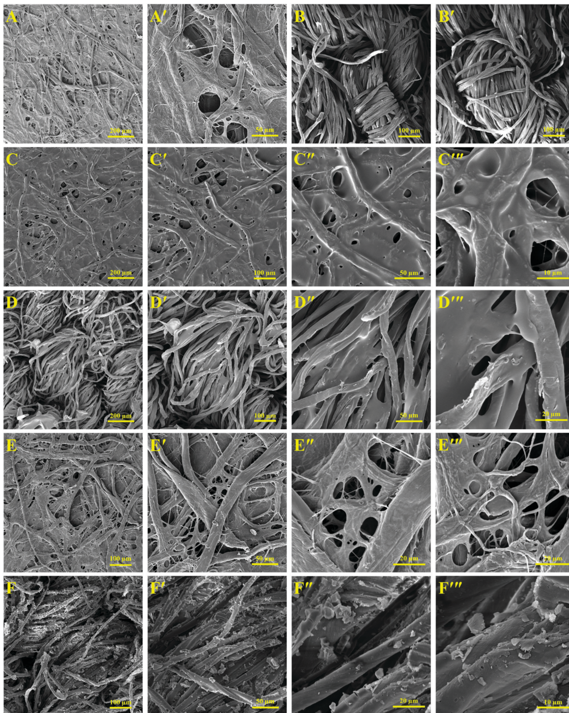
Fig. 9 SEM images of the impregnated cellulosic paper and tissue with the spirocyan-modified latex particles: (A and A') neat cellulose paper, (B and B') neat cotton tissue, (C–C''') impregnated cellulose paper with PBA-SP, (D–D''') impregnated cotton tissue with PBA-SP, (E–E''') impregnated cellulose paper with PMMA-SP, and (F–F''') impregnated cotton tissue with PMMA-SP.
