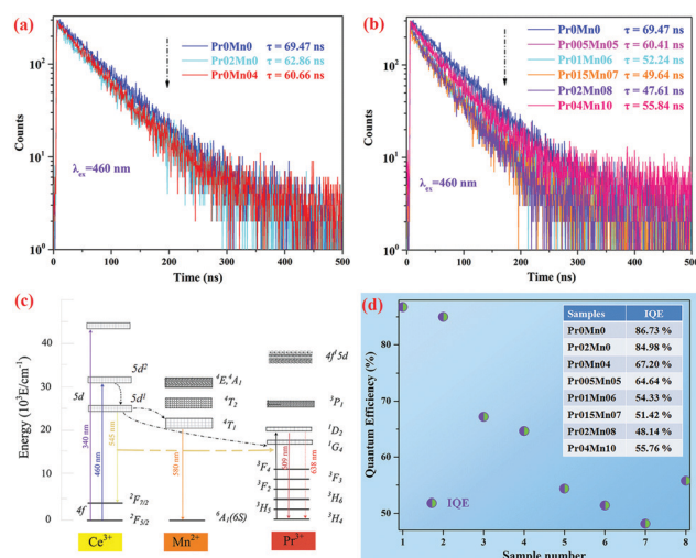
Fig. 8 Fluorescence decay curves: (a) Pr0Mn0, Pr02Mn04. (b) Pr0Mn0, Pr005Mn05, Pr01Mn06, Pr015Mn07, Pr02Mn08, Pr04Mn10. (c) Schematic of the energy transfer process among \text{Ce}^{3+}\text{-Pr}^{3+}\text{-Mn}^{2+} ions. (d) Internal quantum efficiencies (IQEs) of the TCs under 460 nm excitation.
