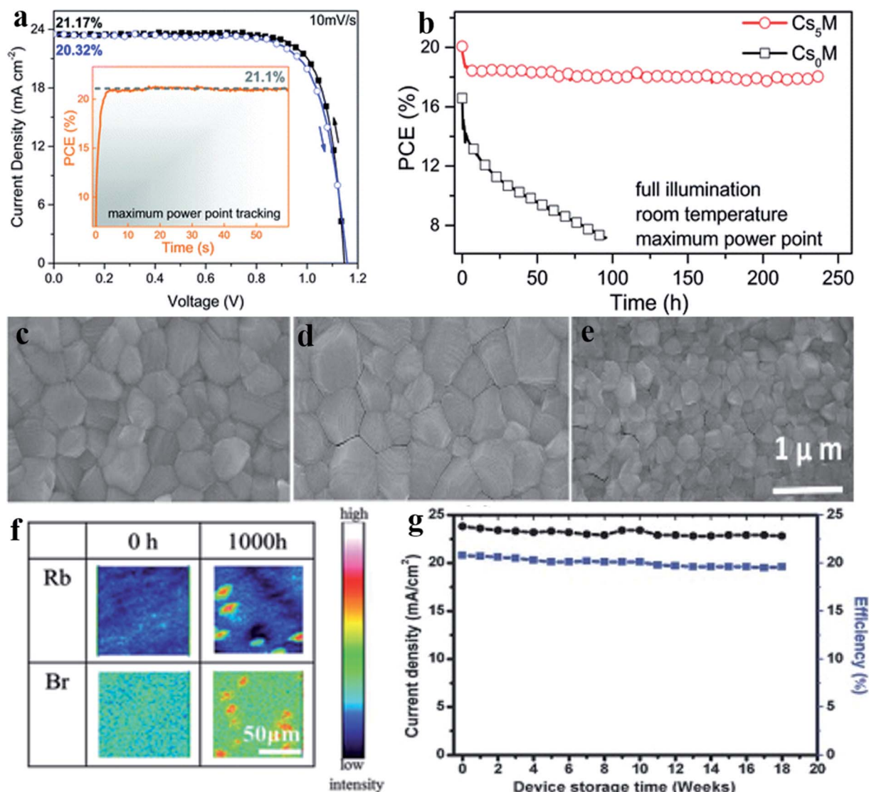
Fig. 10 (a) J-V scan for \text{Cs}_5\text{M} device that shows power conversion efficiency above 21% (b) change in device efficiency with time up to 250 hours of a high-performance \text{Cs}_5\text{M} and \text{Cs}_0\text{M} devices which kept in \text{N}_2 atmosphere at room temperature with constant illumination and maximum power point tracking. Reproduced by permission ref. 89, Copyright 2016 Royal Society of Chemistry. Top view scanning electron microscope images of perovskite thin films made from (c) \text{Cs}_0 , (d) \text{Cs}_5 , (e) \text{Cs}_{10} . Reproduced by permission ref. 88, Copyright 2017 Wiley-VCH Verlag GmbH & Co. KGaA, Weinheim. (f) Top-view TOF-SIMS elemental mapping of the \text{Rb}_{0.05}\text{Cs}_{0.05}\text{FA}_{0.75}\text{MA}_{0.15}\text{Pb}(\text{I}_{0.83}\text{Br}_{0.17})_3 perovskite thin film before and after thermal stress test at 85^\circ\text{C} for 1000 h. Reproduced by permission ref. 90, Copyright 2019 Wiley-VCH Verlag GmbH & Co. KGaA, Weinheim. (g) Current density and efficiency change with device storage time in weeks. Reproduced by permission ref. 88, Copyright 2017 Wiley-VCH Verlag GmbH & Co. KGaA, Weinheim.
