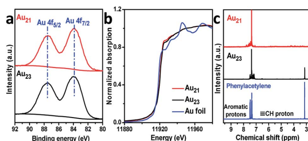
Fig. 5 (a) Au 4f XPS and (b) Au L_{3\text{-edge}} XANES profiles of \text{Au}_{21}(\text{SR})_{12}(\text{Ph}_2\text{PCH}_2\text{PPh}_2)_2 and \text{Au}_{23}(\text{SR})_{16} . (c) The ^1\text{H} NMR spectra of Au-acetylide species.
