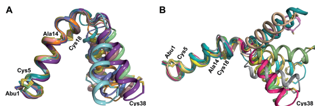
Fig. 13 (A) Superimposition of the 10-structure ensemble of \text{CyLL}_s'' that adopts a more compact organization with an acute angle between helices A and C. (B) Superimposition of the 10-structure ensemble of \text{CyLL}_L'' that adopts a more linear conformation with an obtuse angle between helices A and C.
