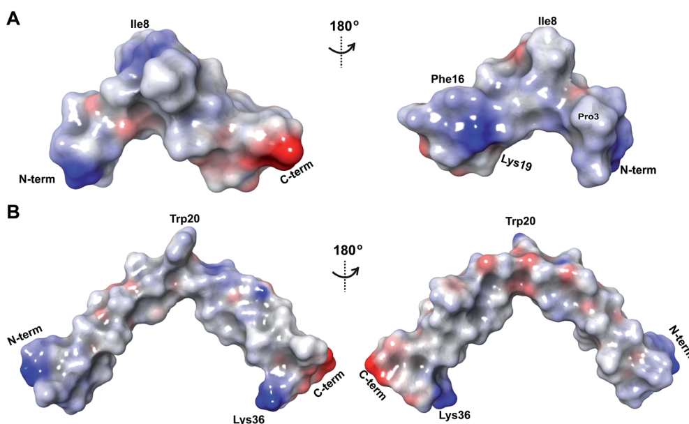
Fig. 14 Electrostatic potential surface maps for (A) \text{CyLL}_s'' and (B) \text{CyLL}_L'' .
