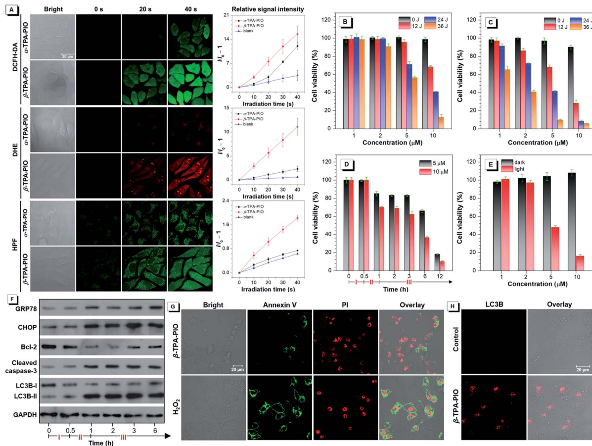
Fig. 6 (A) General ROS, \text{O}_2^{\cdot-} and \text{OH}^{\cdot} generation of \alpha -TPA or \beta -TPA in HeLa cells by using DCFH-DA, DHE and HPF as indicators, respectively, before and after exposure to 405 nm laser irradiation at 1% power with the plot of relative signal intensity of indicators against irradiation time. Data are shown as mean \pm SD ( n = 3 ). Cell viability after treatment with a range of concentrations and irradiation doses using (B) \alpha -TPA-PIO or (C) \beta -TPA-PIO as the PS and white light irradiation of 20 mW \text{cm}^{-2} for 0, 10, 20 or 30 min. (D) Cell viability vs. time during the PDT treatment with \beta -TPA-PIO. (E) Viability of cells after treatment with a range of concentrations without or with white light irradiation of 20 mW \text{cm}^{-2} for 30 min under hypoxic conditions. Cell viability data are shown as mean \pm SD ( n = 6 ). (F) Western blot analysis of various protein expressions vs. time during PDT treatment with \beta -TPA-PIO. (G) Cell apoptosis analysis after treatment by PDT using 10 \mu M \beta -TPA-PIO as the PS (white light irradiation of 20 mW \text{cm}^{-2} for 30 min) and further culturing for 12 h or 880 \mu M \text{H}_2\text{O}_2 for 6 h, by staining with annexin V-Alexa Fluor TM 488 conjugate and PI as the indicator. (H) Immunofluorescence of HeLa cells after treatment with 10 \mu M \beta -TPA-PIO (white light irradiation of 20 mW \text{cm}^{-2} for 30 min) and further culturing for 2 h, using anti-LC3B antibody with an Alexa Fluor ® 488-labeled secondary antibody as an autophagosome marker. Phase I: treatment with \beta -TPA-PIO in the dark for 30 min; Phase II: irradiation with white light of 20 mW \text{cm}^{-2} for 30 min; Phase III: further culturing in the dark.
