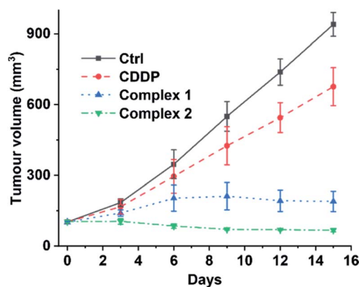
Fig. 9 Volume of A549 tumours in mice treated intravenously with CDDP ( 1.3 \text{ mg}_{\text{Pt}} \text{ kg}^{-1} ), 1, and 2 ( 1.1 \text{ mg}_{\text{Pt}} \text{ kg}^{-1} ) every three days for 15 d.
