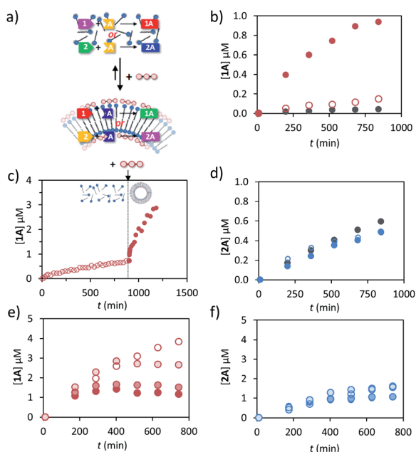
Fig. 3 (a) Schematic representation of the reactions between 1 , 2 and A to give hydrazones 1A and 2A in the untemplated and templated state. (b) Concentration of 1A as a function of time as determined by HPLC when 1 (20 \mu\text{M} ) and A (5 \mu\text{M} ) were added to aqueous buffer at pH 7.0 (grey), a solution of \text{C}_{12}\text{TACN}\cdot\text{Zn}^{2+} (100 \mu\text{M} ) (empty red circles) or a solution of \text{C}_{12}\text{TACN}\cdot\text{Zn}^{2+} (100 \mu\text{M} ) and ATP (200 \mu\text{M} ) (filled red circles). (c) Concentration of 1A as a function of time as determined by HPLC when 1 and A (20 \mu\text{M} ) were added to a solution of \text{C}_{12}\text{TACN}\cdot\text{Zn}^{2+} (100 \mu\text{M} ) and to which ATP (200 \mu\text{M} ) was added after 900 minutes. (d) Concentration of 2A as a function of time when 2 (20 \mu\text{M} ) and A (5 \mu\text{M} ) were added to aqueous buffer at pH 7.0 (grey), a solution of \text{C}_{12}\text{TACN}\cdot\text{Zn}^{2+} (100 \mu\text{M} ) (empty blue circles) or a solution of \text{C}_{12}\text{TACN}\cdot\text{Zn}^{2+} (100 \mu\text{M} ) and ATP (200 \mu\text{M} ) (filled blue circles). (e and f). Concentration of 1A (e)/ 2A (f) as a function of time when 1 (e)/ 2 (f) (20 \mu\text{M} ) and A (20 \mu\text{M} ) were reacted together in the presence of \text{C}_{12}\text{TACN}\cdot\text{Zn}^{2+} (100 \mu\text{M} ), ATP (200 \mu\text{M} ) and increasing concentrations of alkaline phosphatase (0–2 U). General experimental conditions: [HEPES] = 5 mM, pH 7.0, T = 25^\circ\text{C} .
