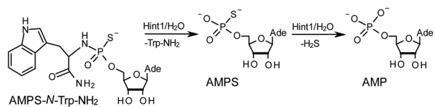
Scheme 3 The HINT1 catalyzed hydrolysis of adenosine-5'- O -(( L -tryptophan amide- N_{\alpha} -yl)-phosphoramidothioate) (AMPS-Trp-NH 2 ), followed by desulfuration of the AMPS intermediate leading to the formation of adenosine-5'- O -phosphate.
