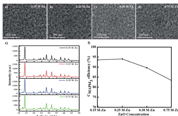
Fig. 6 SEM surface morphologies of the MAPbI 3 perovskite layers fabricated on ZnO ((a) 0.19 M-Zn, (b) 0.25 M-Zn, (c) 0.38 M-Zn, (d) 0.75 M-Zn) over the c-TiO 2 layers under two SDC and three SSIER cycles and (e) the XRD patterns of these MAPbI 3 perovskite layers and (f) the C_{\text{MAPbI}_3} values for various thicknesses of ZnO layers.
