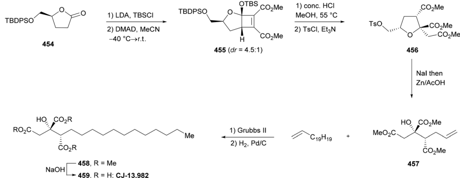
Scheme 110 Synthesis of (-)-CJ-13,982.
