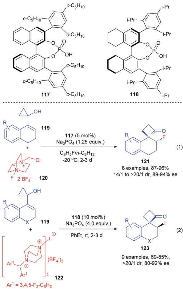
Scheme 36 Asymmetric sulfenylation/semipinacol rearrangement.
