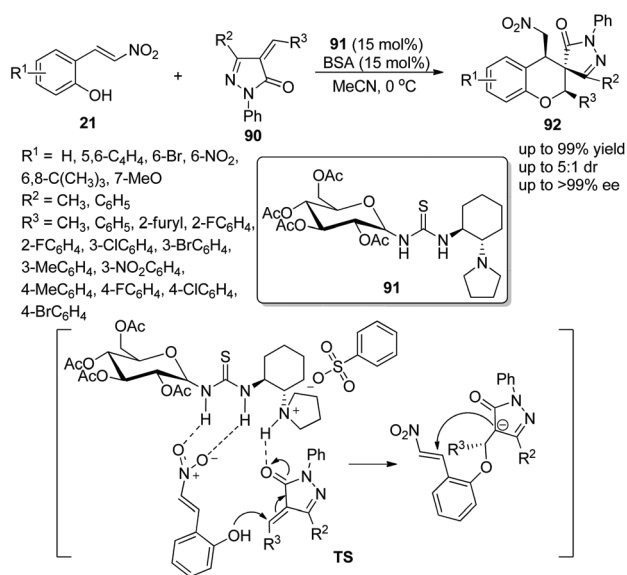
Scheme 32 Oxa-Michael/Michael cascade reaction for the synthesis of chiral spiro benzohydroxyran-pyrazolones.
