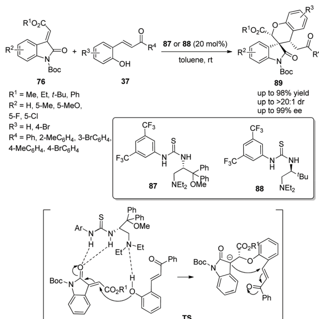
Scheme 31 Oxa-Michael/Michael cascade reaction for the synthesis of chiral spiro benzohydroxyran-oxindoles.
