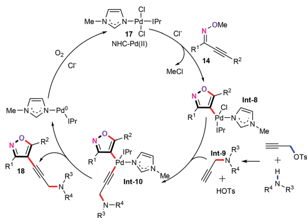
Scheme 8 Plausible mechanism for palladium-catalyzed cascade cyclization/alkynylation.
