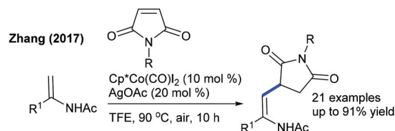
Scheme 44 Coupling of enamides with maleimides.
