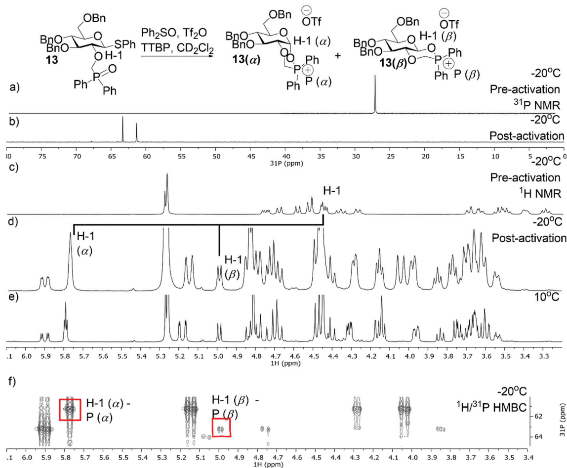
Fig. 3 VT-NMR spectra of the phosphonium ion derived from 13 (a) ^{31}\text{P} NMR spectrum of 13 at -20\text{ }^{\circ}\text{C} in \text{CD}_2\text{Cl}_2 . (b) ^{31}\text{P} NMR of 13 at -20\text{ }^{\circ}\text{C} after the addition of \text{Tf}_2\text{O} . (c) ^1\text{H} NMR spectrum of 13 at -20\text{ }^{\circ}\text{C} in \text{CD}_2\text{Cl}_2 . (d) ^1\text{H} NMR of 13 at -20\text{ }^{\circ}\text{C} after the addition of \text{Tf}_2\text{O} . (e) ^1\text{H} NMR of 13 at 10\text{ }^{\circ}\text{C} . (f) ^1\text{H}/^{31}\text{P} HMBC at -20\text{ }^{\circ}\text{C} .
