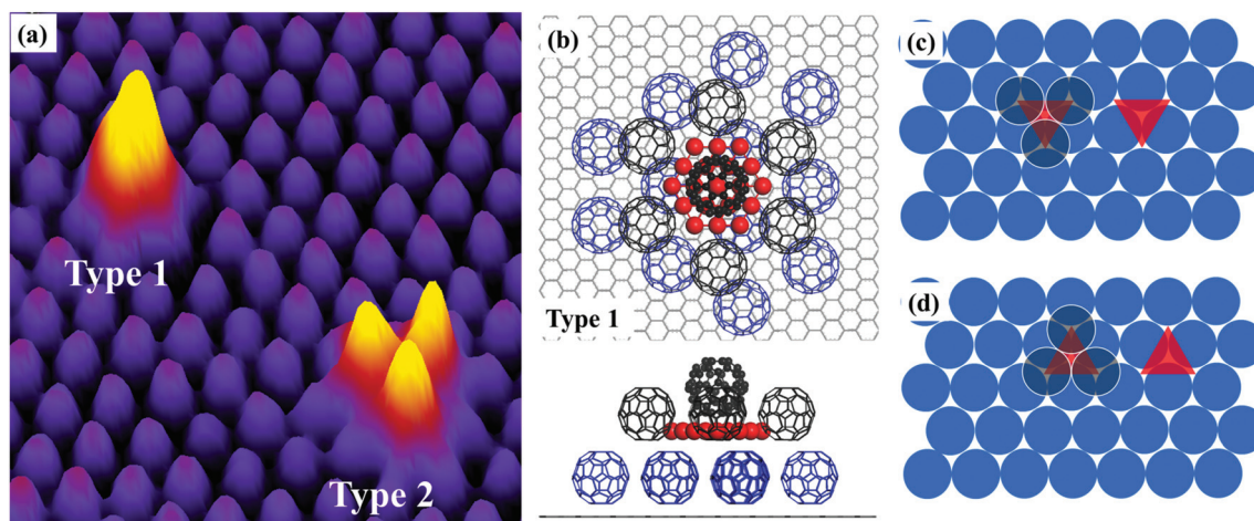
Fig. 5 Structural models of Au clusters trapped between two layers of C 60 . (a) STM image showing two types of raised features. Type I: a single raised C 60 molecule. Type II: a raised C 60 trimer. The C 60 molecules in this image are all in the second layer. (b) Structural model for Au clusters trapped at the tetrahedral interstitial site. (c) Structural model for Au clusters trapped at the octahedral site. (d) Alternative arrangement of the octahedral site. The raised C 60 trimer in (c) has an opposite orientation to that in (d).
