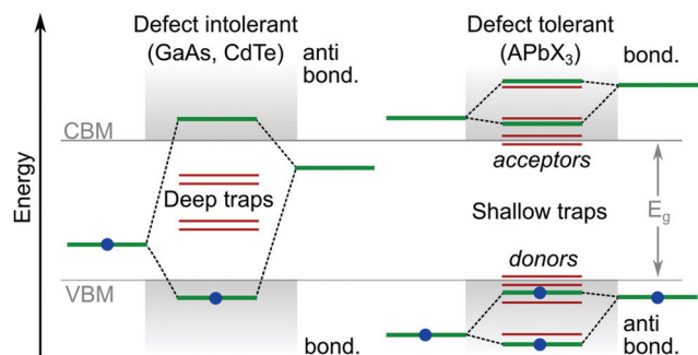
Fig. 4 Comparison of typical trap energies relative to the electronic band structure of traditional defect intolerant compound semiconductors ( i.e. III–V and II–VI varieties) and defect tolerant 43 lead halide perovskite materials. 1,2
