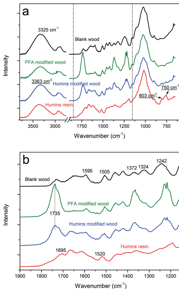
Fig. 1 (a) IR spectra of blank wood (black line), PFA modified wood (green line), humin modified wood (blue line) and humin resins (red line) (a) in the range 3800\ cm^{-1} – 700\ cm^{-1} and (b) zoom on the region 1900\ cm^{-1} – 1100\ cm^{-1} .
