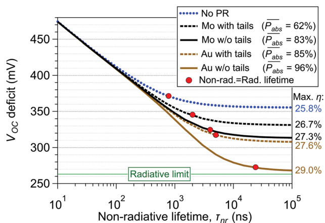
Fig. 4 V_{\text{OC,def}} as a function of non-radiative lifetime for different average reflectance properties at the back, i.e. molybdenum ( R \sim 30\% ) and gold ( R > 90\% ), and no photon recycling consideration (No PR). The maximum achievable efficiency ( i.e. at \tau_{\text{nr}} = 100 \mu\text{s} ) is shown on the right side of the graph.
