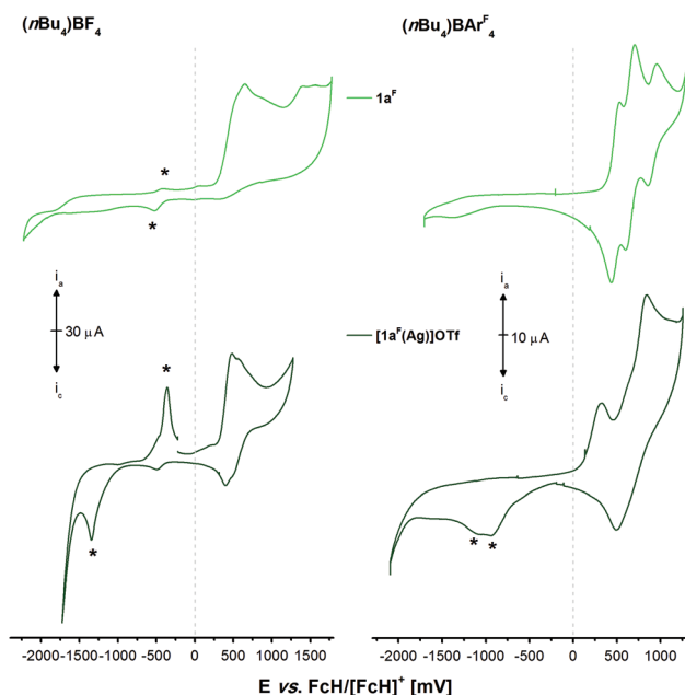
Fig. 9 Cyclic voltammograms of 1 mmol L −1 1a F (light green) and [1a F (Ag)]OTf (dark green) in 0.1 mol L −1 supporting electrolyte solutions (( n Bu 4 N)BF 4 (left) and ( n Bu 4 N)BAr 4 F (right) in CH 2 Cl 2 ). Traces have been recorded at 100 mV s −1 (working electrode: glassy carbon, counter electrode: Pt wire) at room temperature. The second of three cycles are shown and asterisks (*) mark oxidation/reduction events which depend on prior oxidation in the first cycle ( cf. Fig. S66 and S67†).
