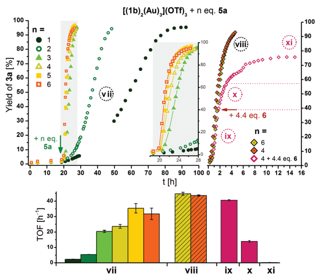
Fig. 13 Top left: Reaction profiles for ring-closing isomerisation of 2 to 3a by [(\mathbf{1b})_2(\text{Au})_3](\text{OTf})_3 (3 mol% Au, [\mathbf{2}]_0 = 60 \text{ mmol L}^{-1} , \text{CD}_2\text{Cl}_2 , 25 °C) oxidised by 1–6 eq. of 5a at the indicated time (arrow). The insert shows a magnified time period, and lines connecting the symbols are for visual guidance only. Top right: Reaction profiles for ring-closing isomerisation of 2 to 3a by [(\mathbf{1b})_2(\text{Au})_3](\text{OTf})_3 (conditions as above), oxidised by four (orange/grape) and six (mustard) eq. of 5a directly before the start of the ^1\text{H} NMR monitoring (viii). To one run (grape), 4.4 eq. of reductant 6 were added at the indicated time (arrow). Reaction phases ix–xi correspond to that run only. For TOF regression plots, s. Fig. S81–S89† referring to reaction phases vii and viii–xi.
