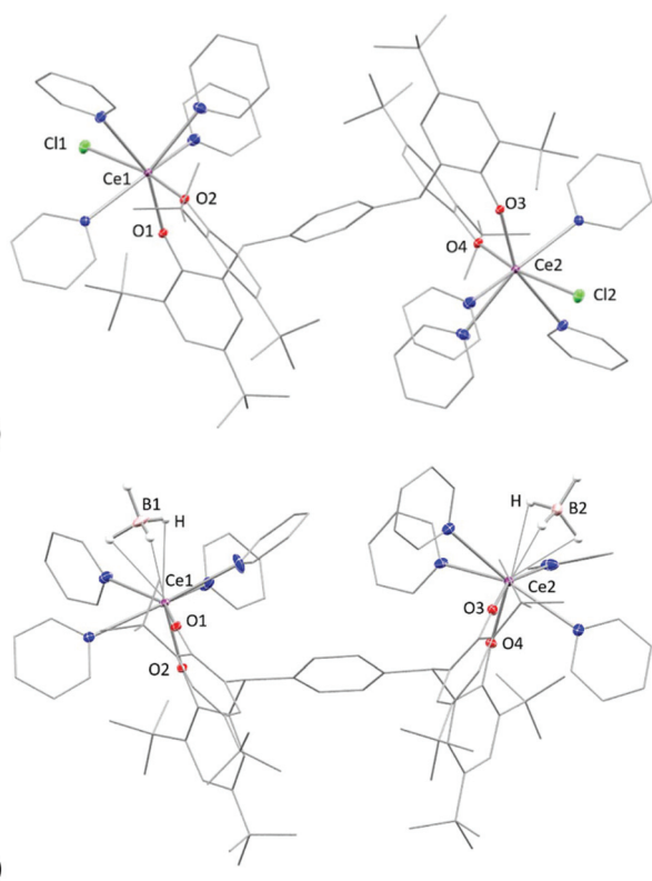
Fig. 3 Solid state structure of complex (a) 3\text{-Ce} (b) 3\text{-Ce-BH}_4 . Thermal ellipsoids are shown at 30% probability. All hydrogen atoms (except for \text{BH}_4 ) and solvents are omitted for clarity. Selected bond lengths in (a): Ln1–Cl1: 2.7789(6)\text{ \AA} (Ce), 2.7601(14)\text{ \AA} (Pr).
