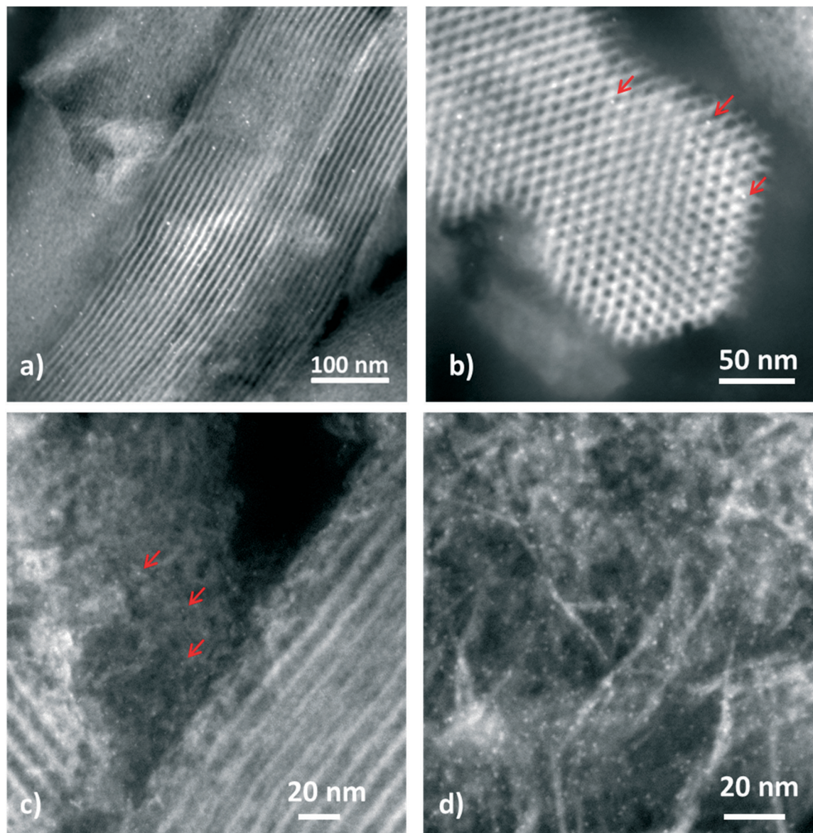
Fig. 1 HAADF-STEM images of a) and b) Pt-Al-SBA-15(20) showing the SBA-15 domains c) and d) Pt- \gamma -Al 2 O 3 /Al-SBA-15(20) showing mainly the \gamma -Al 2 O 3 domains. The arrows point to Pt NPs.
