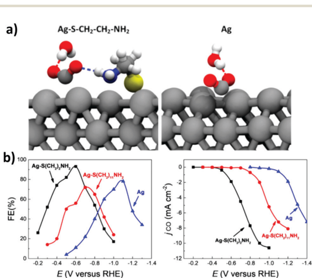
Fig. 31 (a) Chemisorbed \text{CO}_2 on cysteamine-functionalized (left) and on cysteamine-free (right) Ag(111) surface. Only the water molecules directly forming hydrogen bond (slashed line) are shown. The colors are: Ag in silver, C in gray, O in red, N in blue, S in yellow, and H in white. (b) Influence of the alkyl chain length on \text{CO}_2 RR in terms of \text{FE}_{\text{CO}} (left) or j_{\text{CO}} (right) vs. potential. Reproduced with permission from ref. 419. Copyright 2018 American Chemical Society.
