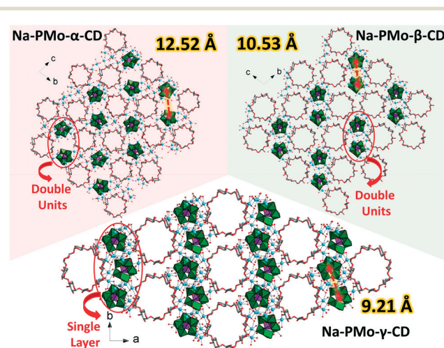
Fig. 4 Structural re-arrangement of MBBs in \alpha -CD MOFs affected by the size of CD analogues.
