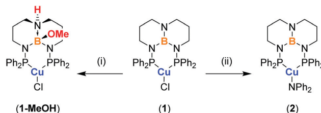
Scheme 1 Structure of ( ^{Ph} TBDPhos)CuCl (1) and synthesis of 1-MeOH and 2. (i) Excess MeOH at RT. (ii) Addition of 1 eq. of HNPPh 2 and KN(SiMe 3 ) 2 in toluene at -78^\circ C .
