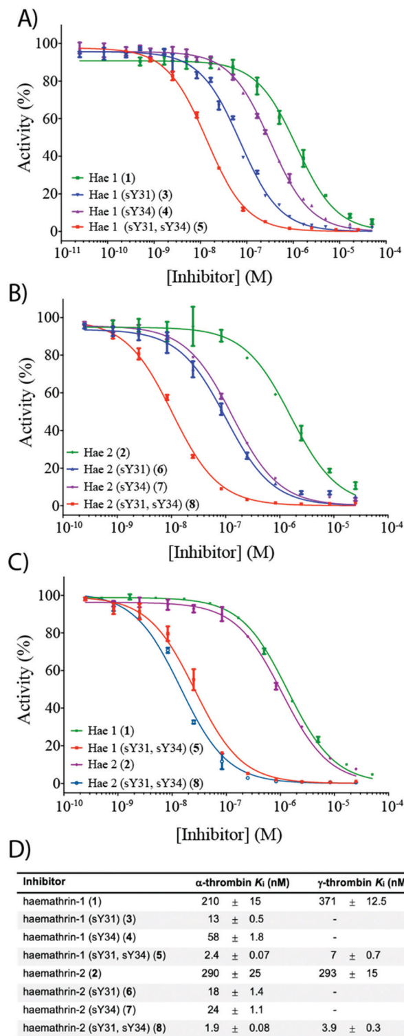
Fig. 2 Dose-response curves for the inhibition of (A) α-thrombin by haemathrin-1 (sulfo)proteins 1 , 3–5 ; (B) α-thrombin by haemathrin-2 (sulfo)proteins 2 , 6–8 and (C) γ-thrombin by unsulfated and doubly sulfated haemathrin-1 and -2 proteins 1 , 2 , 5 and 8 using an amidolytic assay. Error bars represent S.E.M. values; (D) inhibition constants (K i , ±S.E.M.) for haemathrin-1 and -2 (sulfo)proteins. Data were determined by fitting the inhibited steady-state velocities to the Morrison model. 31
