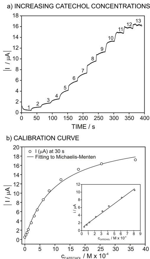
Fig. 3 Calibration graph under the optimized conditions (applied potential of -0.1 V and 1:5 tissue/graphite wt. composition with the particle size of the tissue of 60–250 \mu m for the composition of the electrode material): (a) Recorded dynamic current and (b) corresponding calibration curve. The entire calibration graph was fitted to the Michaelis–Menten equation while the concentration range between 4 \times 10^{-5} and 8 \times 10^{-4} M comprises the linear range of response of the biosensor (inset plot).
