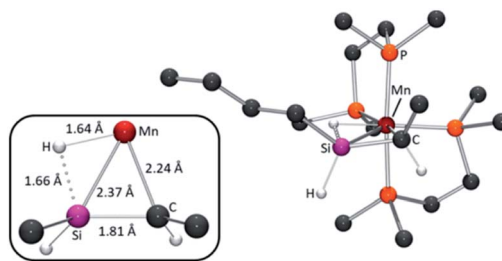
Fig. 4 Calculated structure (ball and stick diagram) for the lowest energy isomer of silene hydride complex [(\text{dmpe})_2\text{Mn}(\textit{n}\text{BuHSi}=\text{CHMe})] ( 6^{\text{Bu,H}} ). All hydrogen atoms have been omitted for clarity except those on Mn or the Si=C unit. The inset shows a top-down view of the Mn silene hydride core, with selected bond distances.
