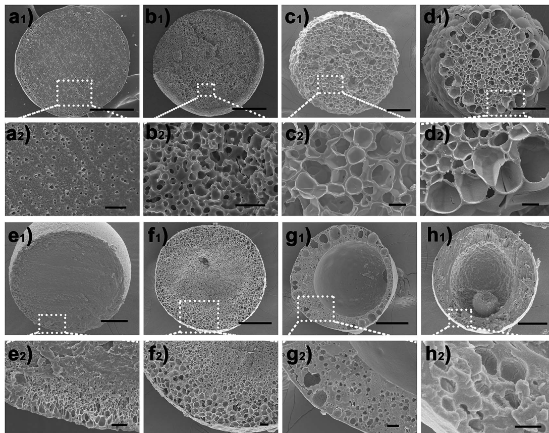
Fig. 5 (a–h) SEM images of diverse emulsion structures induced by judicious choosing of phase separation conditions. (a) Sea-island structure, (b) bicontinuous structure, (c and d) multicompartment structure, (e) anisotropic structure, (f) gradient structure, (g) double emulsion structure, and (h) multiple emulsion structure. Scale bars are 100 \mu\text{m} ( a_1 – h_1 ) and 10 \mu\text{m} ( a_2 – h_2 ).
