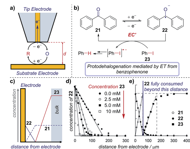
Fig. 22 (a) Schematic of an SECM set-up, where the distance ( d ) between the substrate and tip electrodes can be changed to measure concentrations in solution. The concentration profile of species in the mediated reduction of iodobenzene (b), measured by Amatore et al. using SECM. (c) Schematic of concentration profiles. (d) Concentration profile of 22 with varying equivalents of 23, measured by changing the distance ( d ) between the two electrodes. (e) Comparative concentration profile of various species in solution. (c–e) Adapted with permission from ref. 75. Copyright 2001 John Wiley and Sons.
