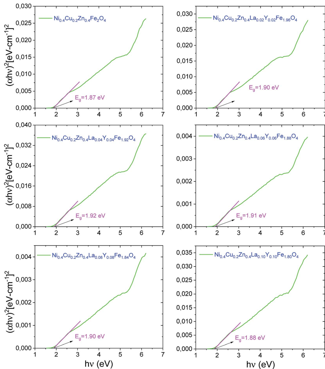
Fig. 6 Tauc plots and extrapolated direct E_g data of \text{Ni}_{0.4}\text{Cu}_{0.2}\text{Zn}_{0.4}\text{La}_x\text{Y}_{1-x}\text{Fe}_2\text{O}_4 ( x = 0.00 - 0.10 ) NPs.
