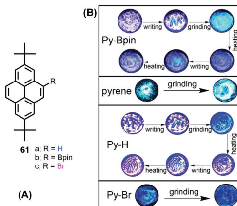
Fig. 39 Structures and images of mechanochemical experiments involving pyrene 1 , Py-Bpin ( 61b ), Py-H ( 61a ) and Py-Br ( 61c ). Reproduced from ref. 97.
