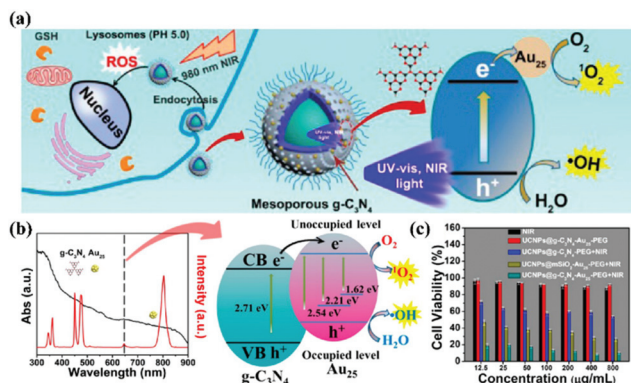
Fig. 7 Improving the excitation light conditions of g-CN optimizes PDT. (a) g-CN combined with UCNP changes the excitation source to near-infrared light and can be combined with the Jinnai cluster to improve the effect of PDT. (b) g-CN and Au 25 have overlapped absorption and luminescence, both of which effectively absorb the light emitted by UCNP. The difference in the energy levels between g-CN and Au 25 can expand the transition of electrons, convert O 2 to O 2 - and convert H 2 O to OH - . (c) When g-CN are combined with Au 25 , the photodynamic effect is significantly improved. Significant differences can be obtained through biotoxicity testing. Reproduced with permission. 67 Copyright 2017, American Chemical Society.
