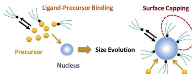
In this manuscript, we investigated the possible mechanisms leading to the focusing and defocusing of colloidal nanoparticle size distribution during the synthesis. We used in situ SAXS to measure the evolution of size, size distribution and concentration of Pd colloidal nanoparticles during synthesis. Using population balance modeling (PBM), we accounted for different possible nucleation and growth pathways and predicted the evolution of the particle size distribution. In addition, we systematically studied the effect of continuous nucleation on the size distribution and how size focusing could be achieved under the condition where nucleation overlaps with the nanoparticle growth. In order to describe the size focusing observed experimentally, our PBM results provide evidence for growth rate constant that strongly depends on ligand coverage. Specifically, we demonstrate that ligand surface coverage plays
