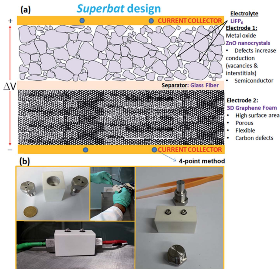
Fig. 1 (a) The superbat design consisting of four basic components. Advanced functional electrodes: 3D graphene foam and ZnO nanocrystals, separator: glass fiber, and electrolyte: 1 M \text{LiPF}_6 in \text{EC}/\text{MC} = 50/50 . (b) The homemade capacitor mounting system.
