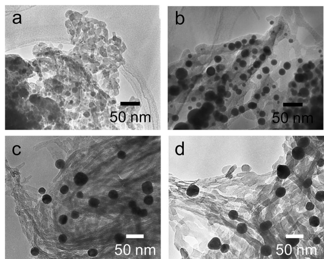
Fig. 2 TEM images of (a) D-, (b) L- \text{Ag@SiO}_2\text{-500} and (c) D-, (d) L- \text{Au@SiO}_2\text{-500} .
