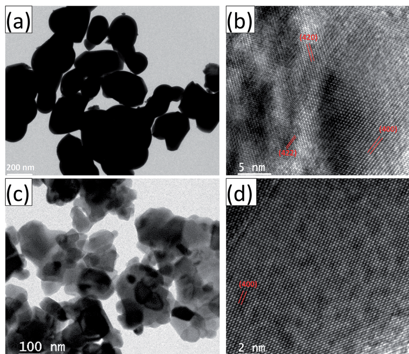
Fig. 5 (a) and (b) are the HRTEM and high-magnification images, respectively, of polycrystalline YIG, x = 0.0 ; (c) and (d) are the HRTEM and high-magnification images, respectively, of preferred (400) oriented single-crystalline Ce-YIG, x = 2.0 .
