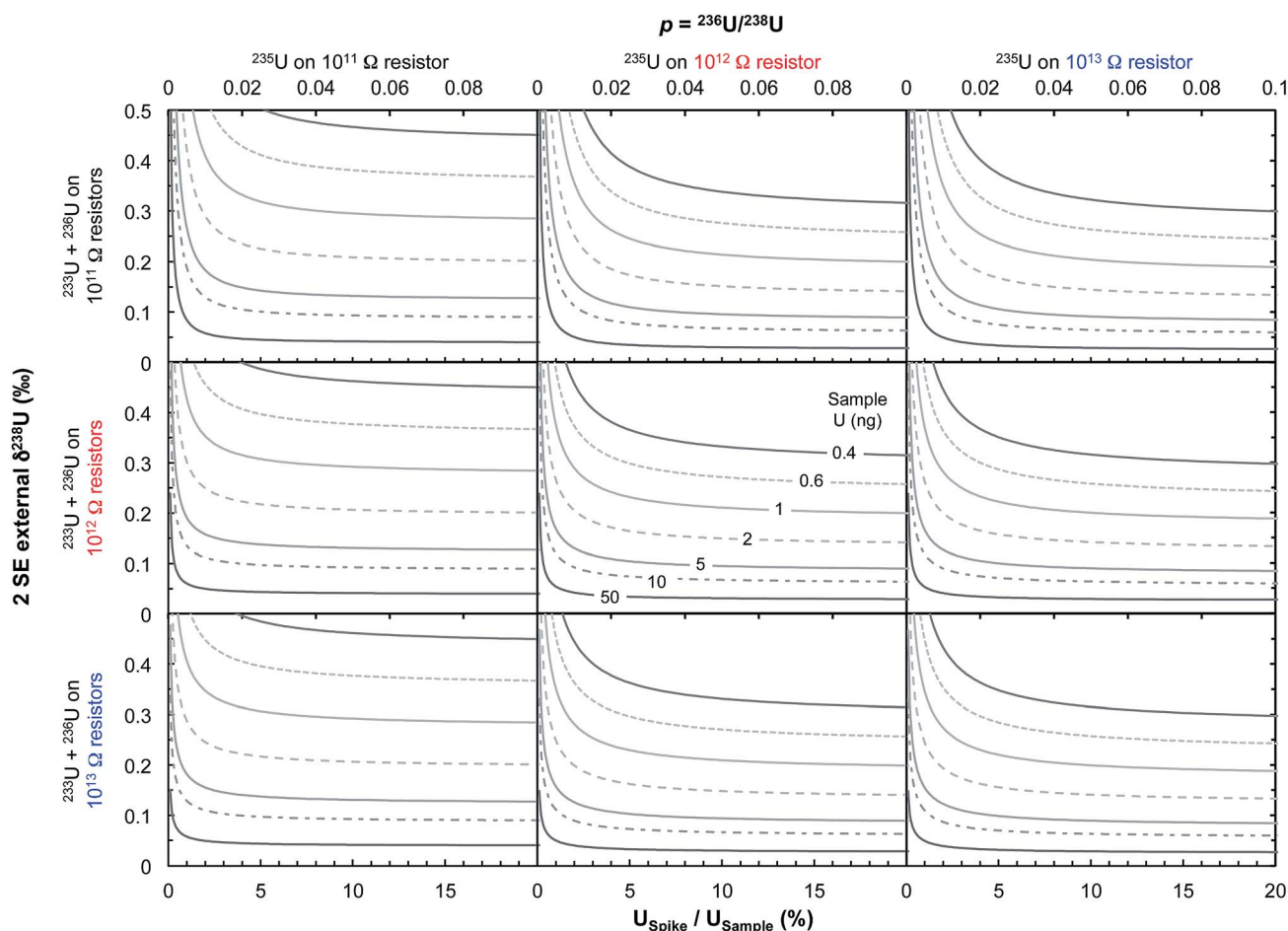
Fig. 12 Theoretical limit on \delta^{238}\text{U} values uncertainty (2 SE external) achievable on Neptune MC-ICPMS plotted as a function of the sample spiking level (bottom x-axis, U_{\text{Spike}}/U_{\text{Sample}} ; top x-axis, parameter p from eqn (2), which relates the number of ions of ^{236}\text{U} and ^{238}\text{U} as: n_6 = p n_8 ). The various curves represent different amounts of total U measured (in ng). Uncertainties are calculated using eqn (2), assuming ^{235}\text{U} is measured at 10 V with a 10^{11} \Omega resistor, and each cycle of 4.192 s consumed 0.072 ng of U. Left, center and right panels assume that ^{235}\text{U} is measured using, respectively, a 10^{11} , 10^{12} or 10^{13} \Omega resistor, with the top, center and bottom row assume that the spike isotopes ( ^{233}\text{U} and ^{236}\text{U} ) are measured using, respectively, 10^{11} , 10^{12} or 10^{13} \Omega resistors, respectively. For small U loads, optimal precision can be achieved using U_{\text{Spike}}/U_{\text{Sample}} ratio of \sim 8 –10% (where uncertainties plateau) and by measuring ^{235}\text{U} in a 10^{12} or 10^{13} \Omega resistor.
