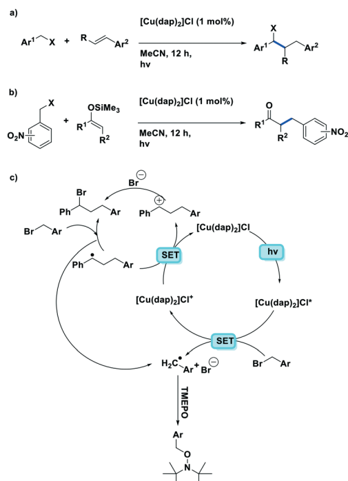
Fig. 16 ATRA of benzyl halides to aryl olefins. ATRA reaction of electron-deficient benzyl halides with silyl enol ethers.
