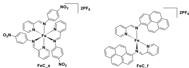
Fig. 49 Chemical structures of iron complexes FeC x which are active photoinitiators.
