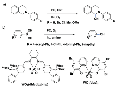
Fig. 38 a) Oxidative cyanation of tertiary amines photocatalyzed by WO 2 (dhfcdbz bmp) and WO 2 (dbp) 2 (where R = C 6 H 5 instead of Br); b) oxidative hydroxylation of aryl boronic acids photocatalyzed by WO 2 (R-dbp) 2 where R = C 6 H 5 .
