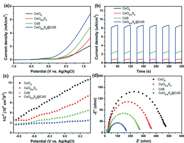
Fig. 5 (a) Linear sweep voltammetry and (b) photocurrent response measurements of the \text{CeO}_2 , \text{CeO}_{2-x}\text{S}_x , \text{CdS} and \text{CeO}_{2-x}\text{S}_x @ \text{CdS} samples under visible-light irradiation ( \lambda > 420 \text{ nm} ) and at a voltage of 0.4 V. (c) Mott–Schottky plots and (d) EIS Nyquist plots of the \text{CeO}_2 , \text{CeO}_{2-x}\text{S}_x , \text{CdS} and \text{CeO}_{2-x}\text{S}_x @ \text{CdS} samples.
