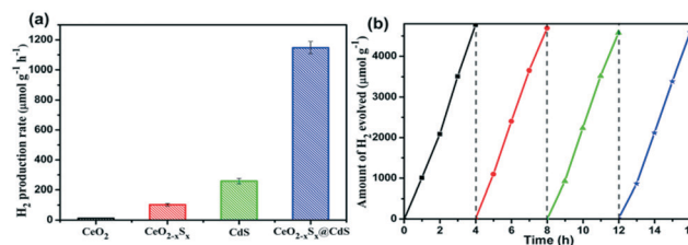
Fig. 6 (a) Comparison of the \text{H}_2 evolution rate of \text{CeO}_2 , \text{CeO}_{2-x}\text{S}_x , \text{CdS} and \text{CeO}_{2-x}\text{S}_x @ \text{CdS} photocatalysts and (b) stability test of \text{H}_2 evolution for \text{CeO}_{2-x}\text{S}_x @ \text{CdS} under visible-light irradiation ( \lambda > 420 \text{ nm} ).
