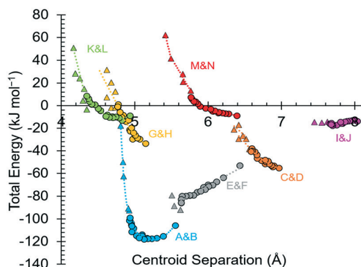
Fig. 8 Molecular interaction energies of contacts A–N as a function of centroid separation. Circles represent phases I to II ( P2_12_12_1 ), and triangles represent phase III ( P2_1 ). The dotted lines have no functional significance and are meant to guide the eye.
