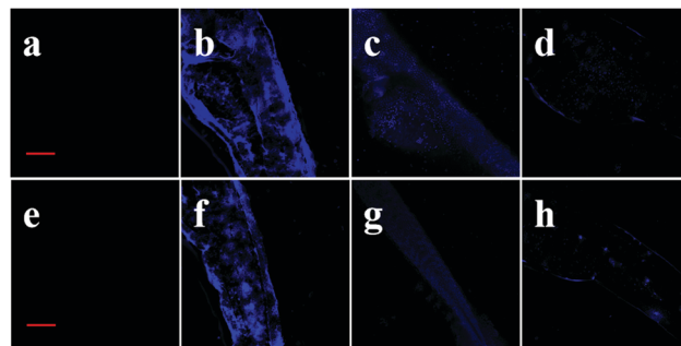
Fig. 4 Fluorescence images of TYR in a living 3-day-old zebrafish (yolk sac and tail): (a and e) zebrafish only (control); (b and f) zebrafish treated with probe 1 (10 \mu\text{M} ) for 3 h; (c and g) zebrafish were pre-incubated with 100 \mu\text{M} kojic acid for 1 h and treated with probe 1 (10 \mu\text{M} ) for 3 h; (d and h) zebrafish were pre-incubated with 200 \mu\text{M} kojic acid for 1 h and treated with probe 1 (10 \mu\text{M} ) for 3 h. Scale bar = 200 \mu\text{m} .
