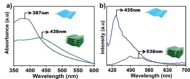
Fig. 4 UV-vis (a) and emission (b) spectra of bulk TTA-DFP COFs (green line) and exfoliated TTA-DFP CONs (blue line) dispersed in water at room temperature, \lambda_{\text{ex}} = 375 \text{ nm} .
