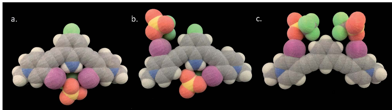
Fig. 8 3D prints generated from the crystal structures (vdW radii) of disordered G2XBme^{2+} \cdot 2OTf^{-} the bidentate (a) and S conformations (b) and G1XBme^{2+} \cdot 2OTf^{-} in the W conformation (c).
